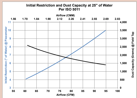
G052829 Straight Outlet
