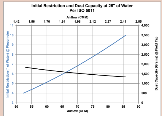
G052742 Straight Outlet
