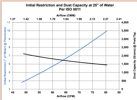
G052741 90° Outlet
