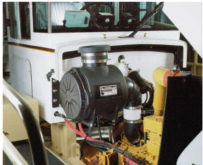
The EPG Air Cleaner, which fits neatly under the hood, has RadialSeal™ Sealing Technology that delivers a reliable seal in rugged environments and quick filter change-out.
