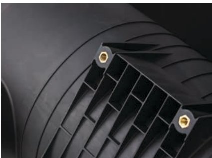
Built-in mounting brackets on air cleaner body eliminate the need for mounting bands.
